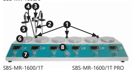
SBS-MR-1600/1T
