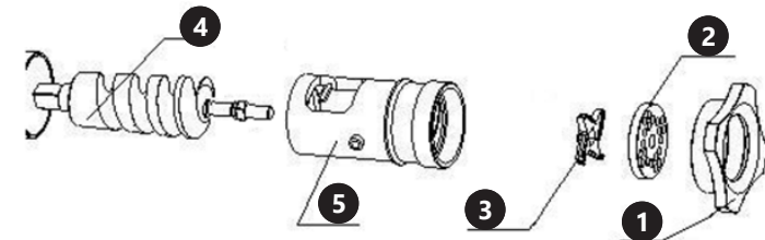
Fig. 6 Modelos RCFW I20PRO y RCFW 220PRO
